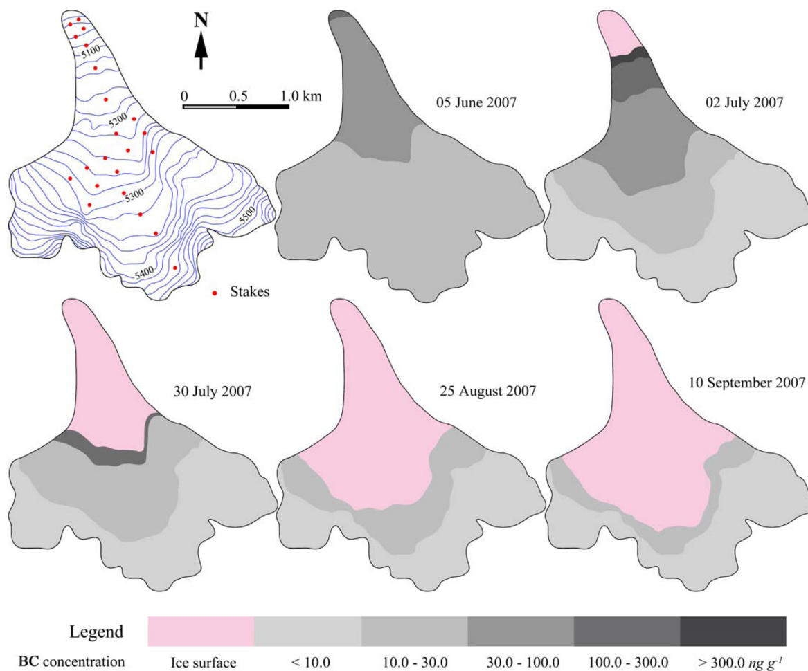
Fig. 4. Topography and calculated BC concentration on a glacier adjacent to the Zuoqiupu that was staked at the indicated locations to measure snow depth throughout the 2007 melt season. Calculated concentrations assume that the annual BC amount measured at the summit is distributed uniformly through the remaining snow depth; i.e., the BC is not carried away by melt water.
