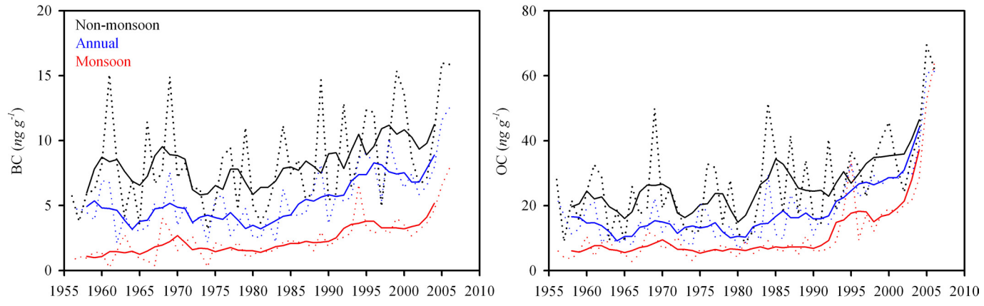
Fig. 3. BC and OC concentrations in the Zuoqiupu ice core for the monsoon (June–September) and nonmonsoon (October–May) seasons, and for the annual mean.
